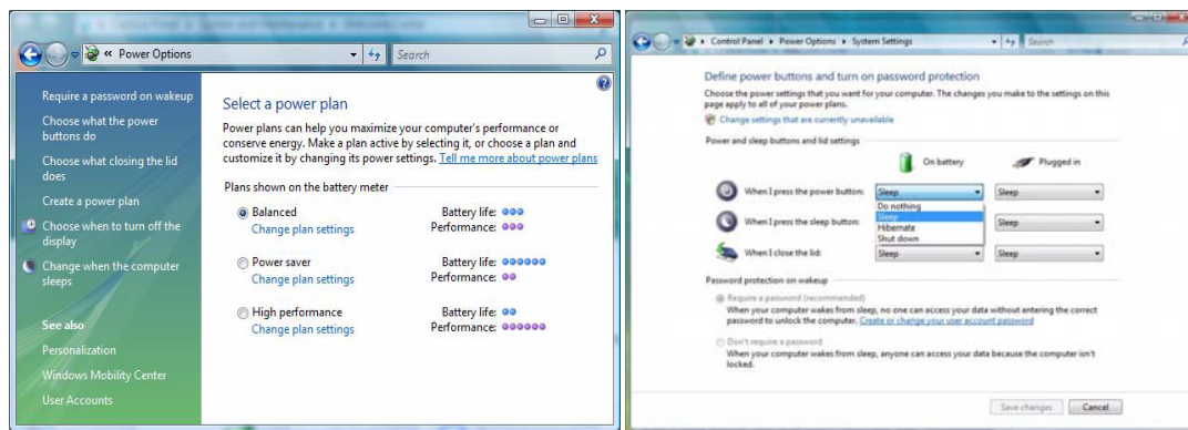
Figure 11 - Power Options
