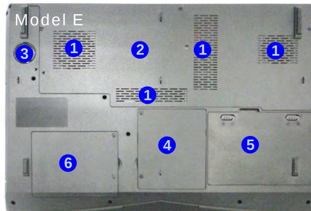
Figure 13 Bottom Views (Models D & E)
